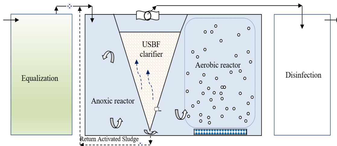
Figure 1. USBF bioreactor of Le Meridien Saigon Hotel.
