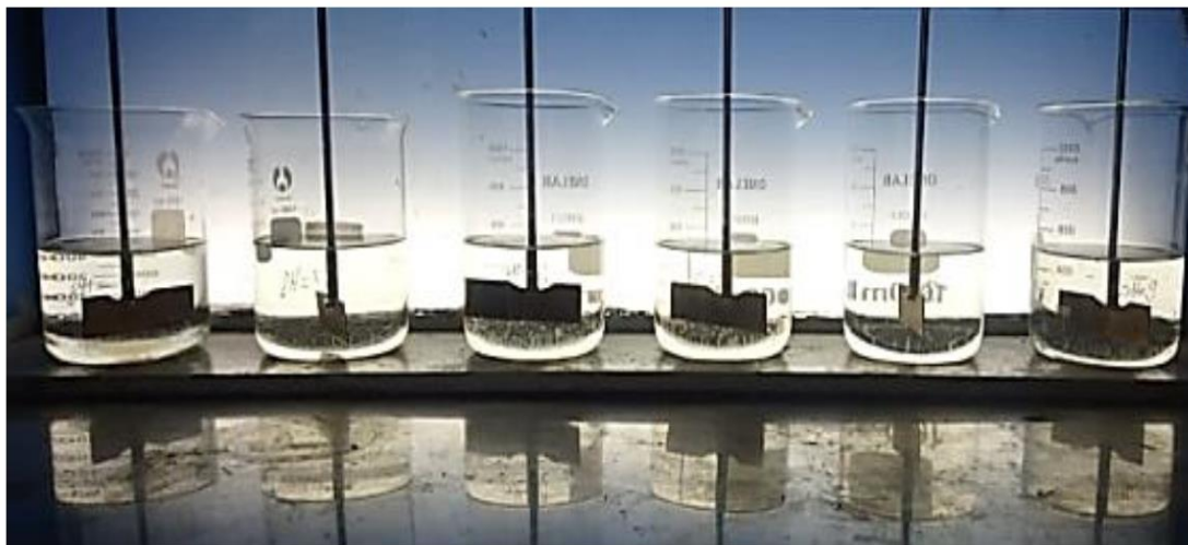
Figure 2. Jar-test procedure.
