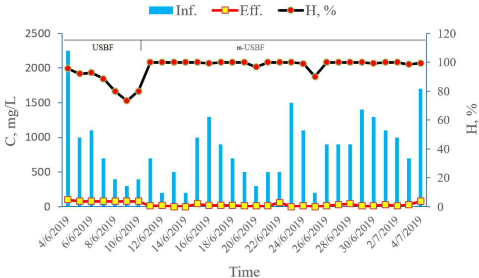
Figure 3. Suspended solids (SS) removal.
