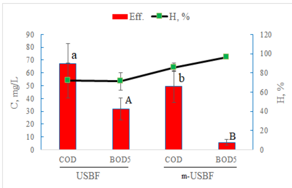
Figure 5. Comparing COD and BOD 5 removal efficiencies.
